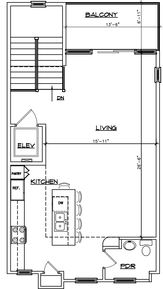
THIRD FLOOR PLAN 1/4"=1'-0"
