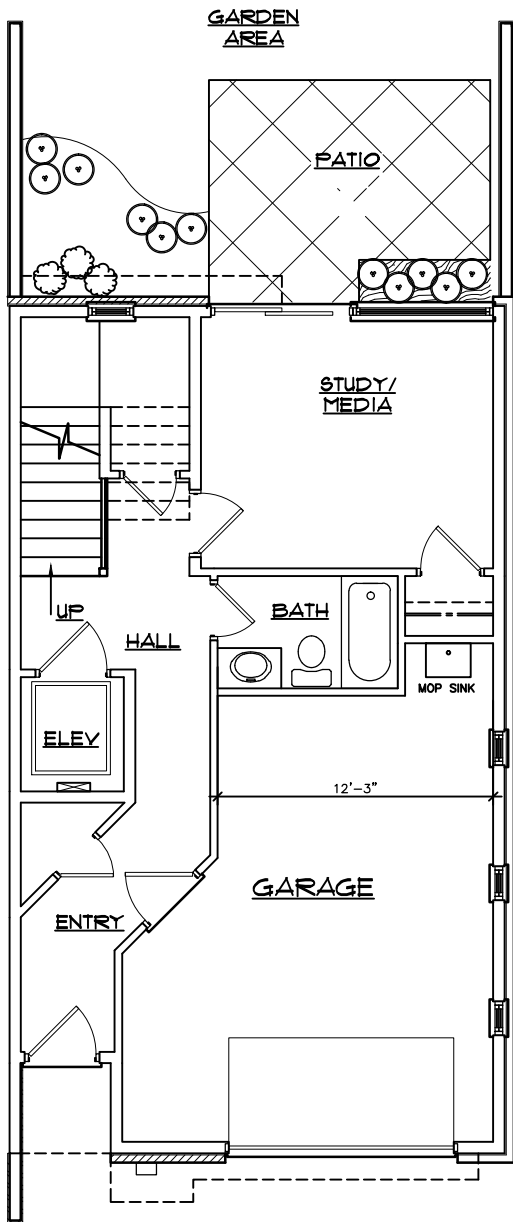
FIRST FLOOR PLAN 1/4"=1'-0" UNIT B
