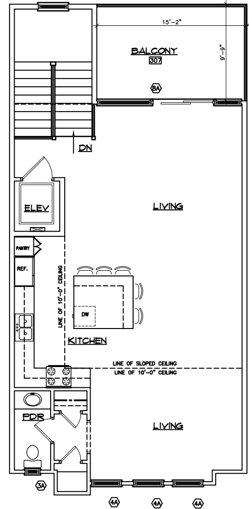
THIRD FLOOR PLAN 1/4"=1'-0"
