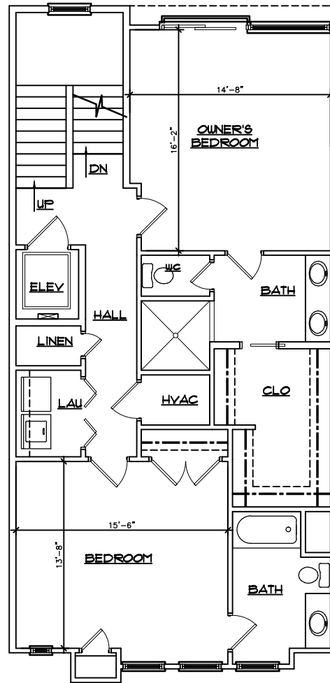
SECOND FLOOR PLAN 1/4"=1'-0"
