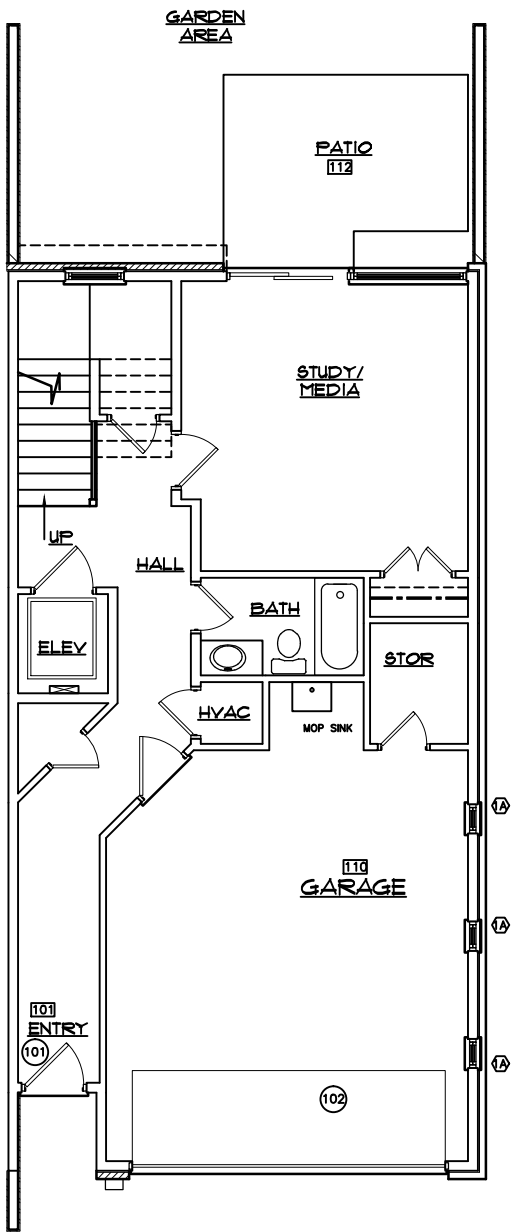
FIRST FLOOR PLAN 1/4"=1'-0" UNIT A
